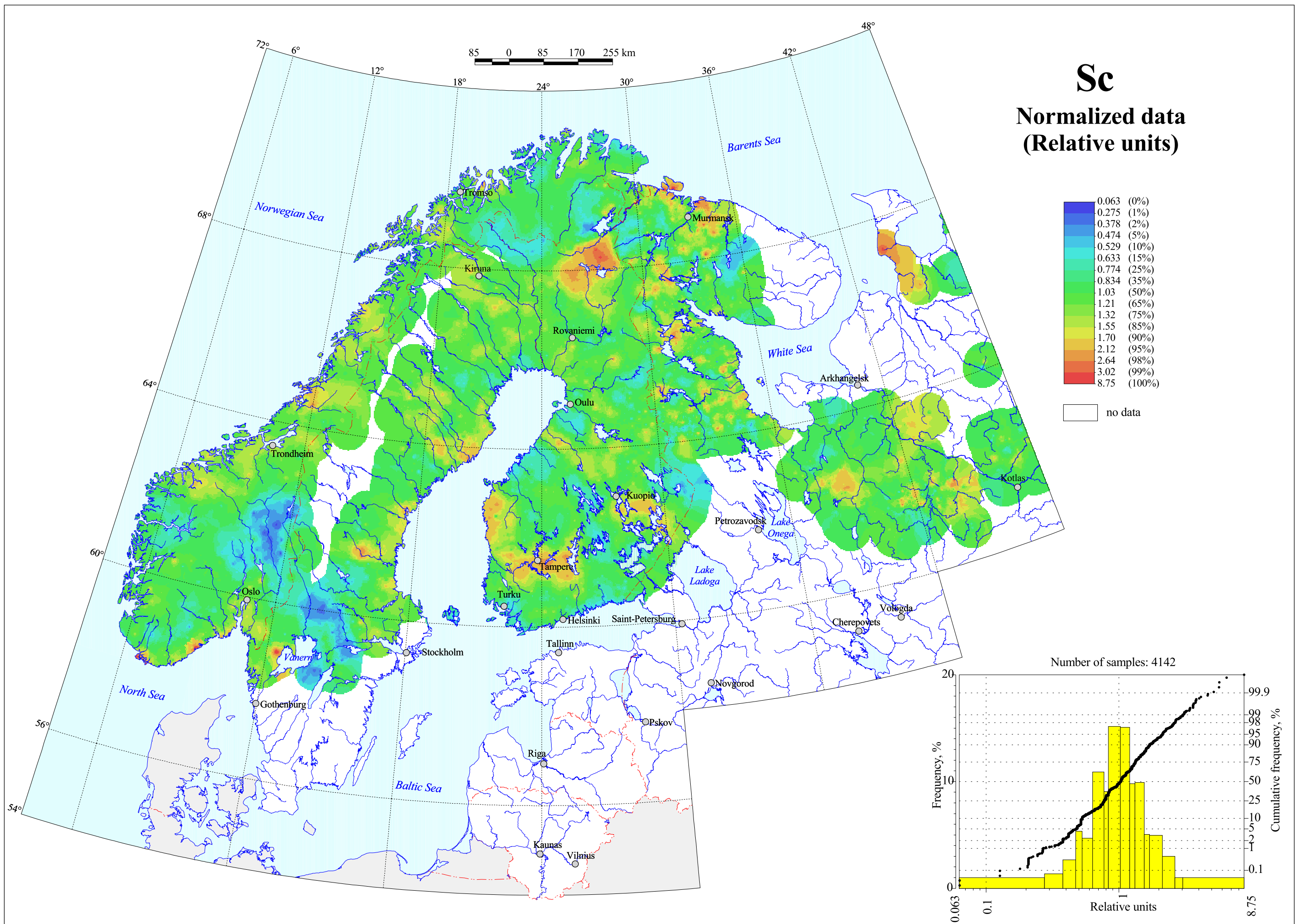
Scandium in Till, Grain Size <0.06 mm
